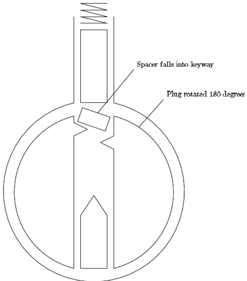
Figure 9.9: Spacer or driver can enter keyway
