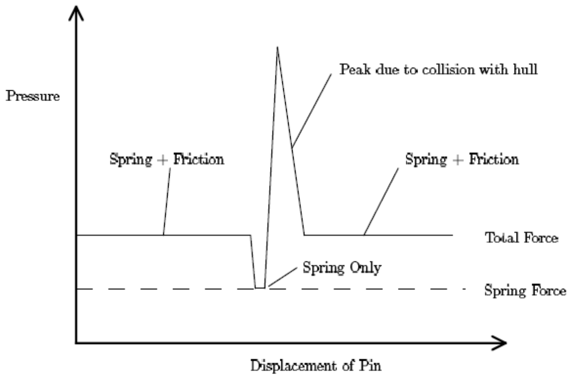
Figure 5.5: Pressure required to move pins
