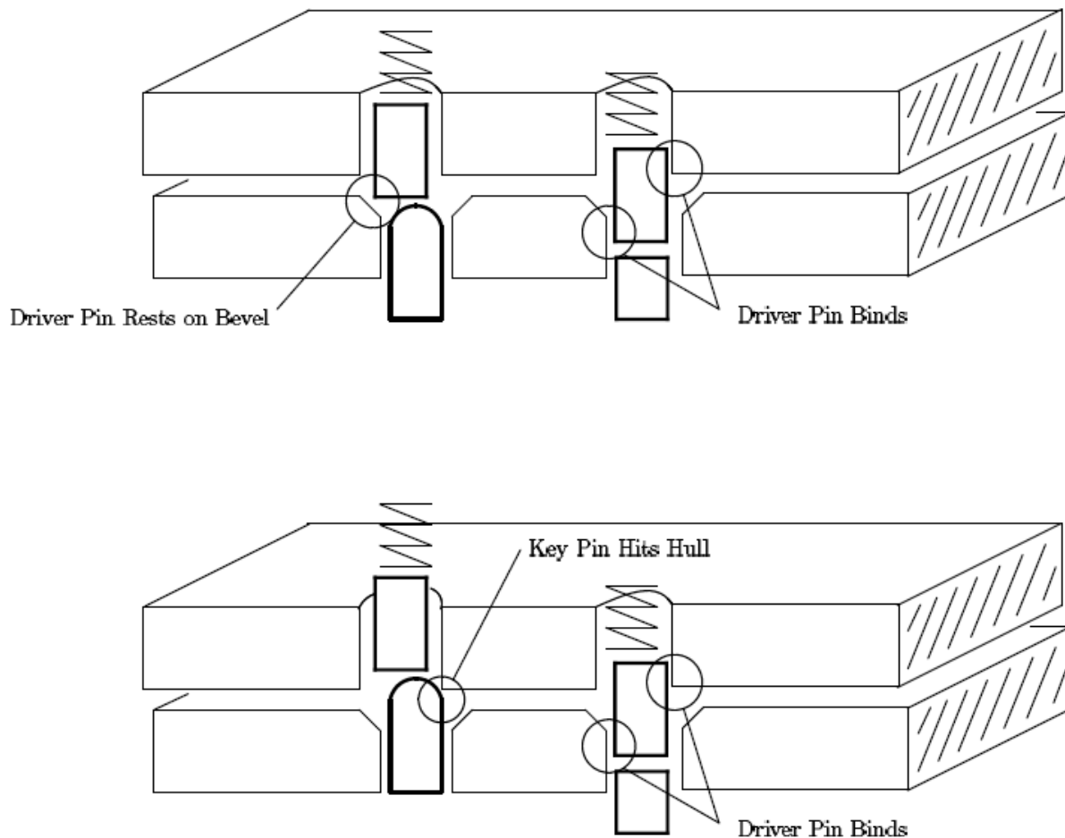
Figure 9.4: Bevelled plug holes and rounded key pins
