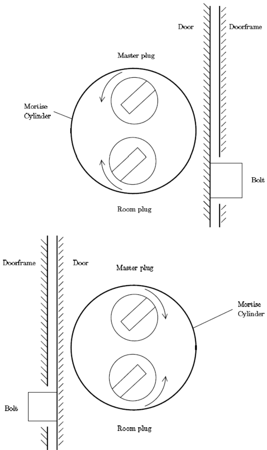
Figure 9.1: Direction to turn plug
