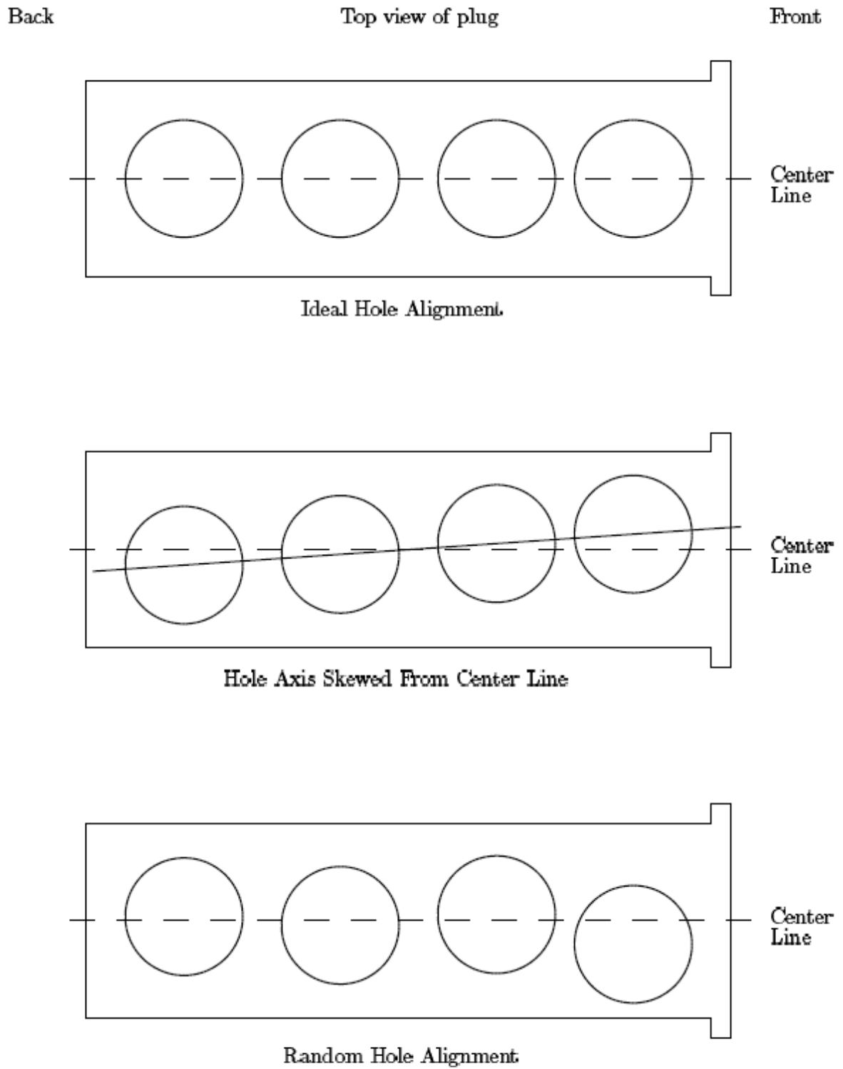
Figure 6.2: Alignment of plug holes
