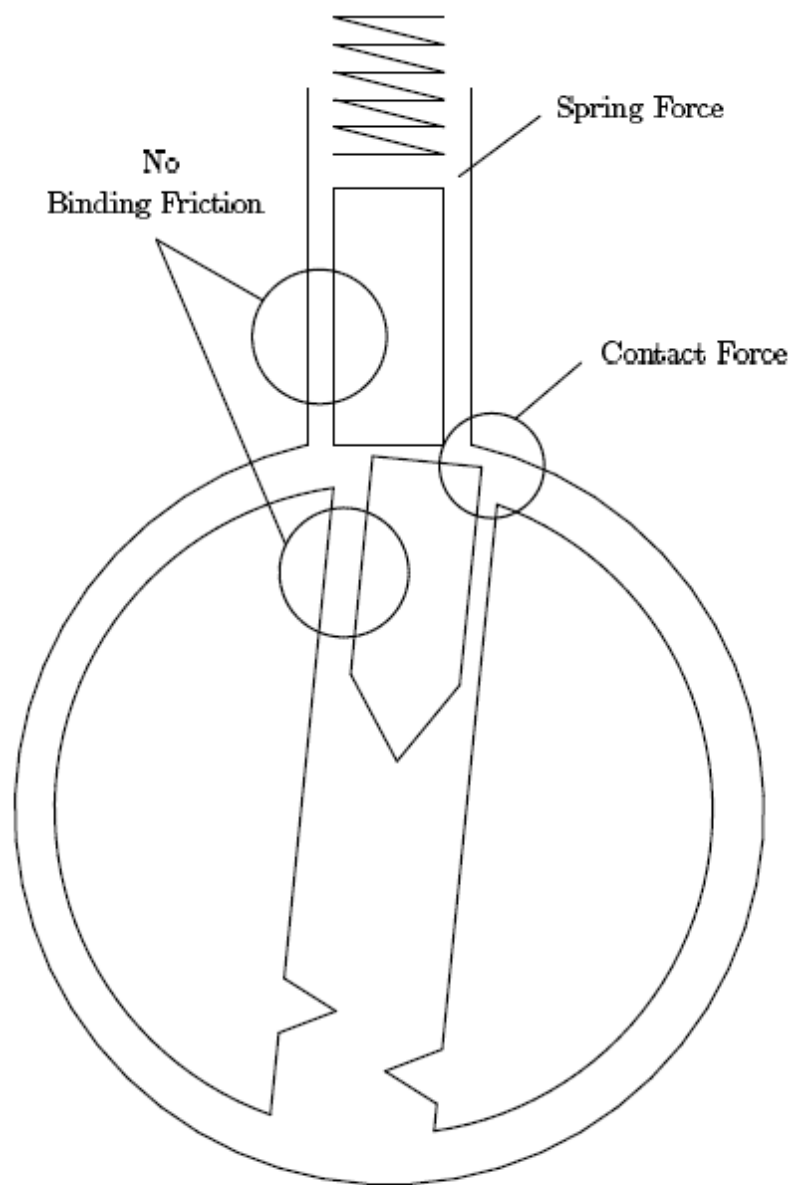
Figure 5.3: Pins at the sheer line
