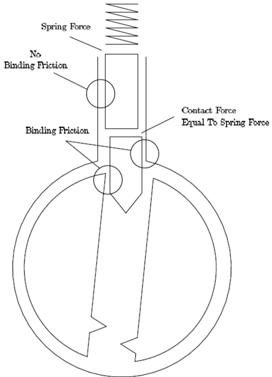
Figure 5.4: Key pin enters hull
