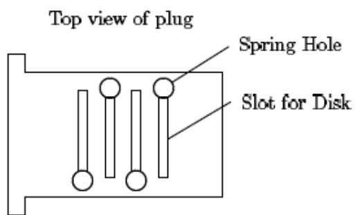
Figure 9.10: Workings of a disk tumbler lock
