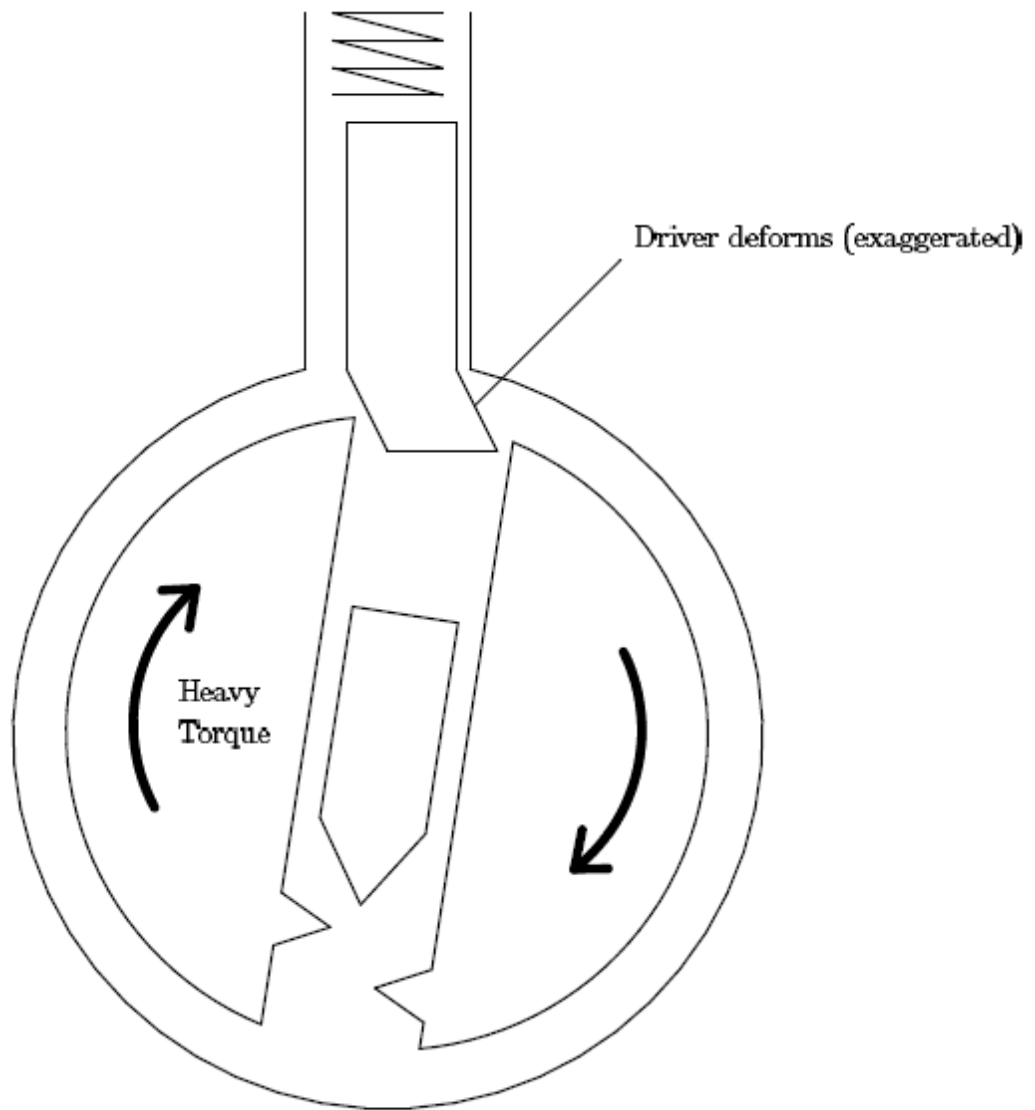
Figure 9.2: Driver pin false set by elastic deformation
