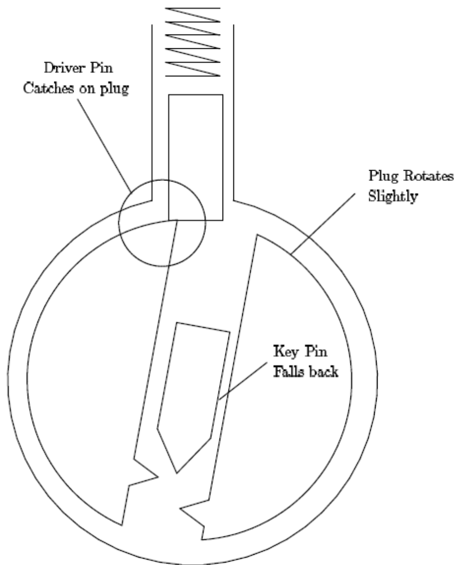
Figure 6.1: Driver pin catches on plug
