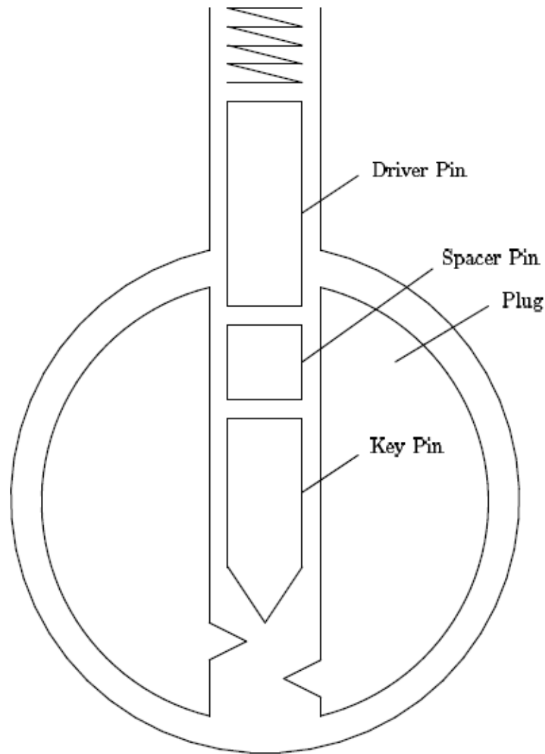
Figure 9.8: Spacer pins for master keying
