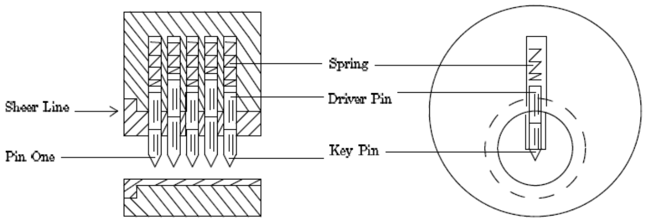
Figure 2.1: Workings of pin tumbler locks
