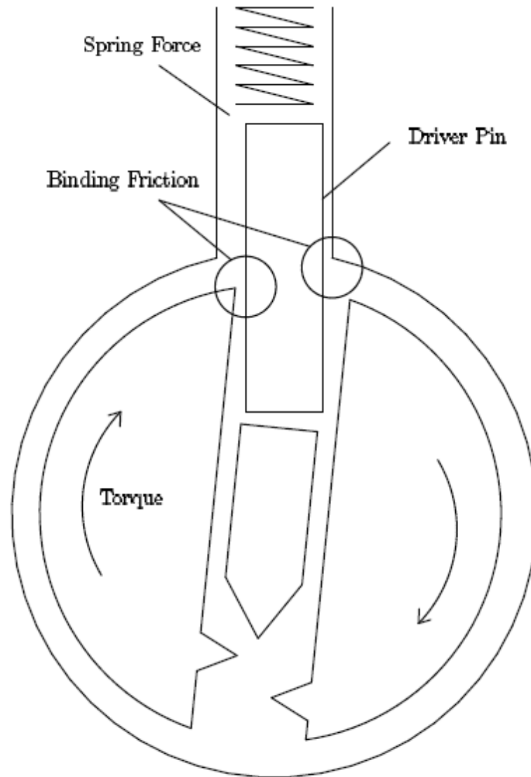
Figure 5.2: Binding in the pin-column model
