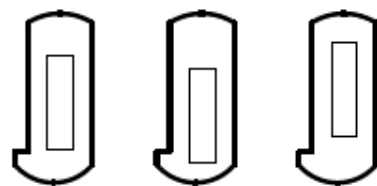
Figure 9.10: Workings of a disk tumbler lock
