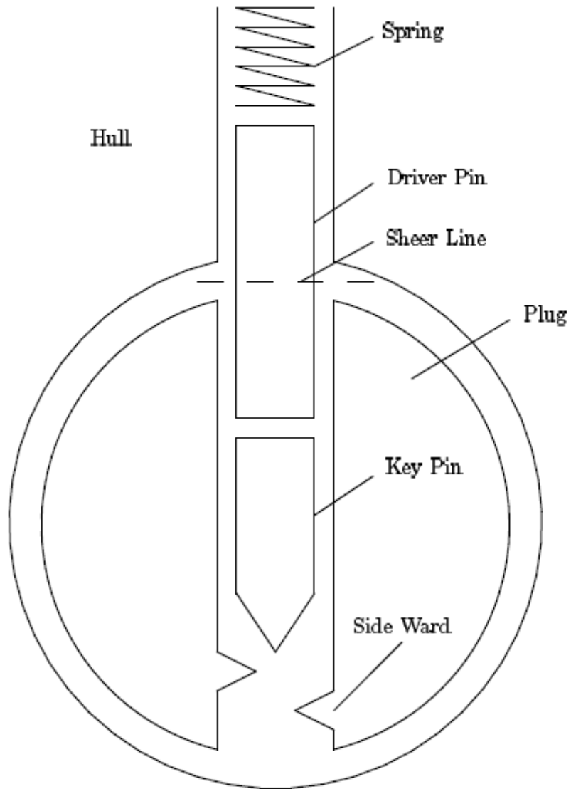
Figure 5.1: The pin-column model
