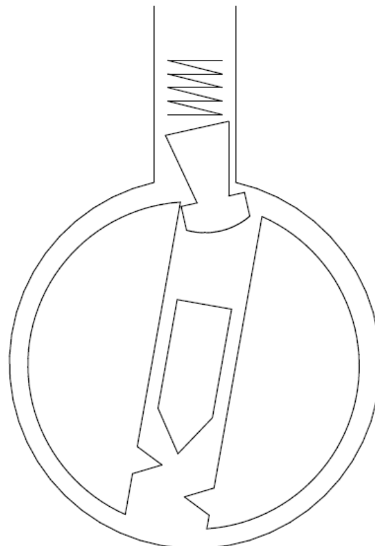
Figure 9.7: Mushroom, spool and serrated driver pins
