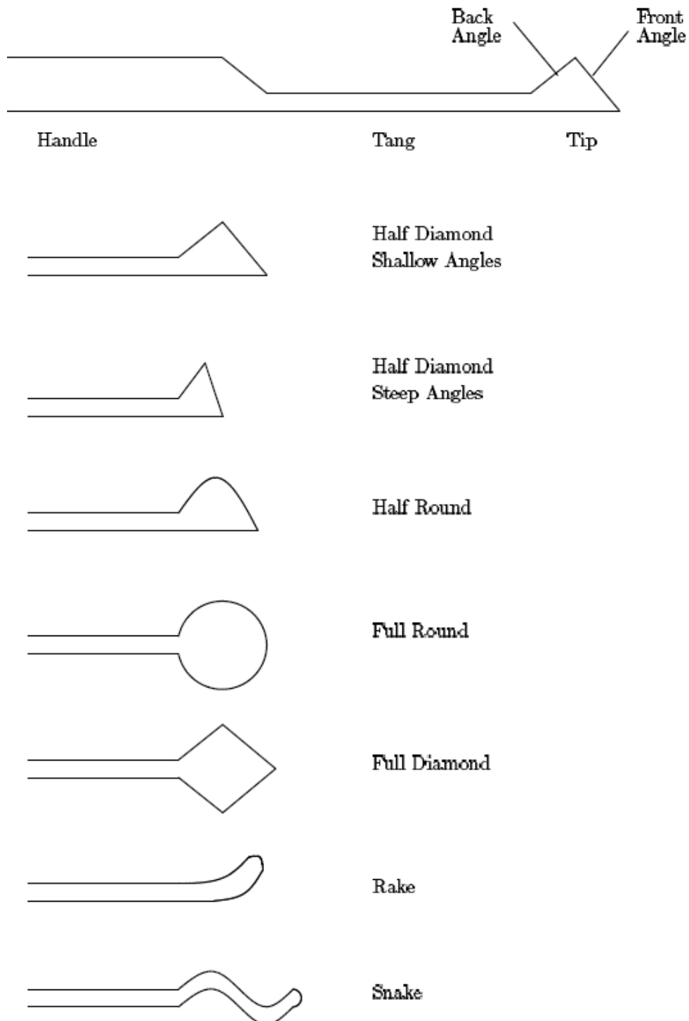
Figure A.1: Selection of pick shapes
